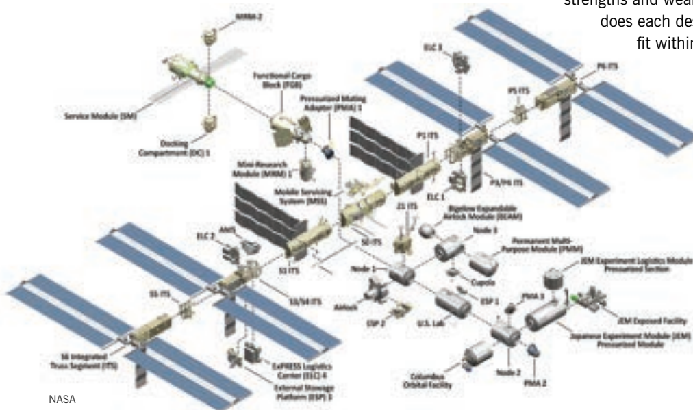
Diagram of the parts of the International Space Station
